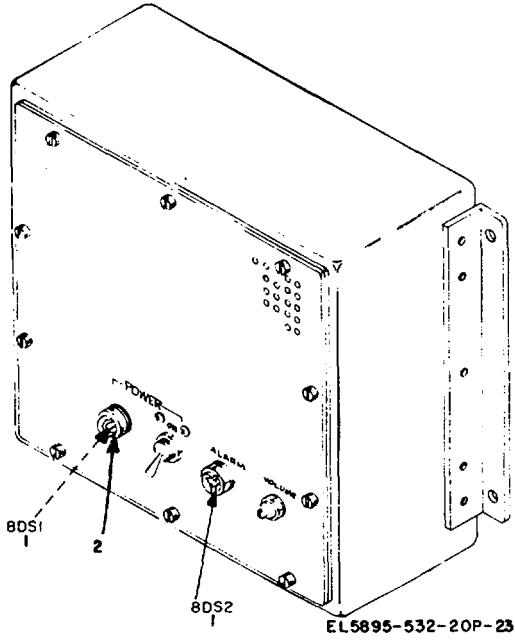
Figure 23. Alarm-Monitor BZ-162/TPX-46(V)-8.
