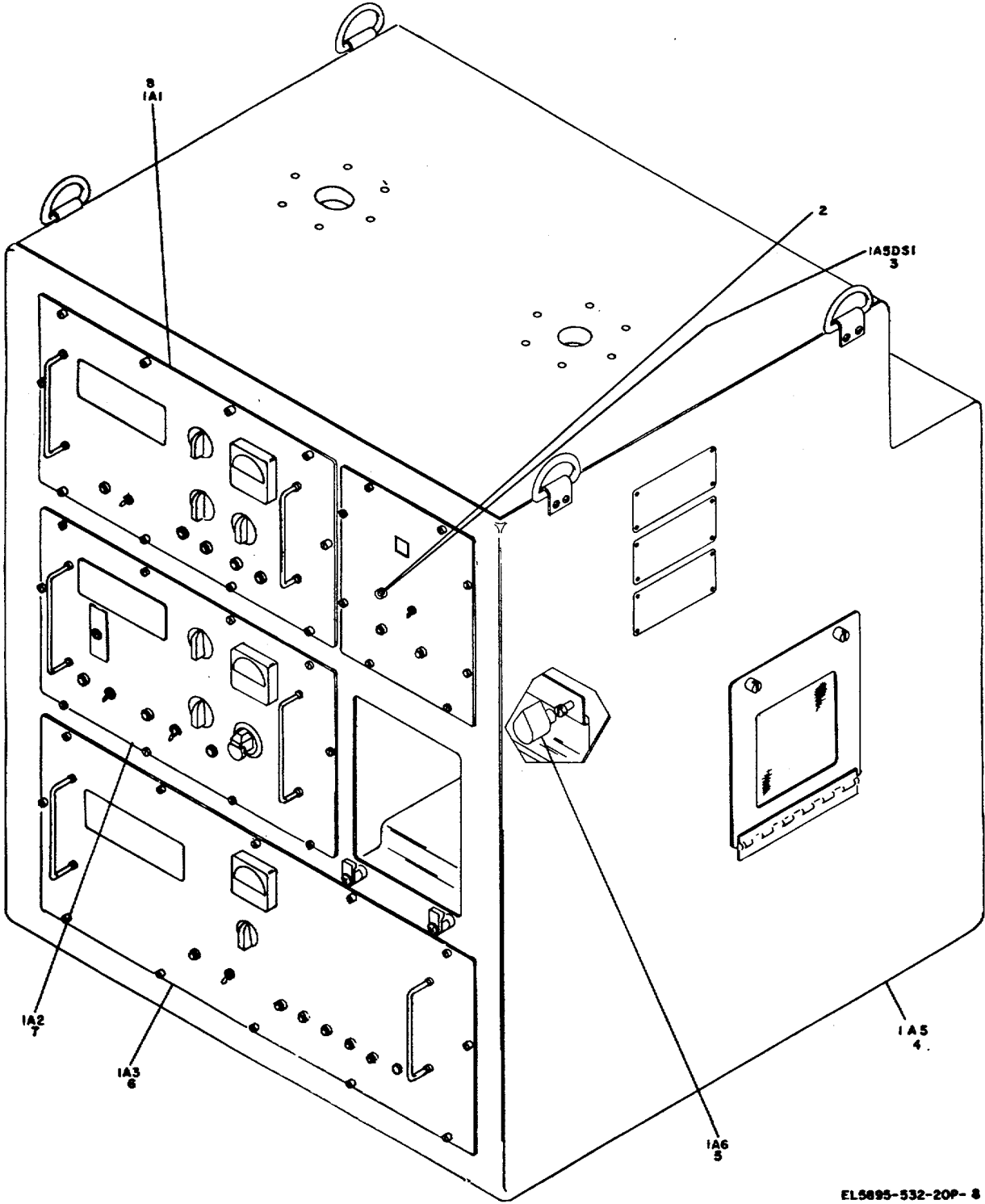
Figure 8. Coder-Decoder Group OX-7(V)1/TPX-46(V)-1.
